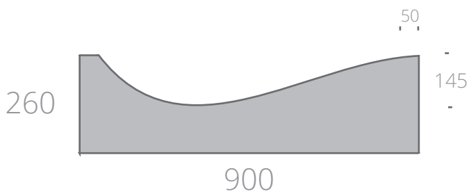
Off Set 900mm Dish Channel
