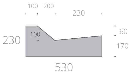
Low Profile Kerb and Channel
