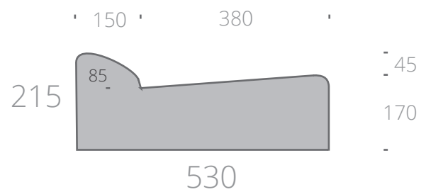
Low Profile Kerb and Channel
