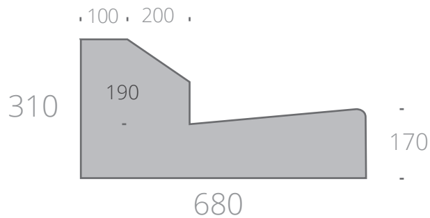
Mountable Kerb and Channel
