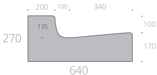
Large Kerb and Channel
