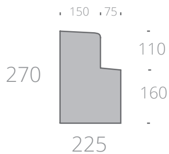
Kerb And Nib CCC SD 602
