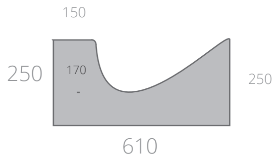
Hillside Kerb and Channel
