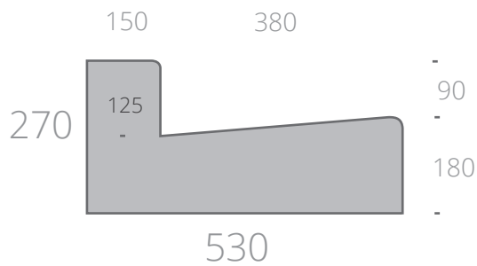
Kerb and Channel
