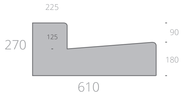
City Kerb and Channel
