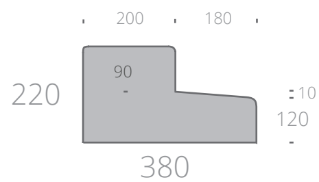
Pegasus Kerb & Nib
