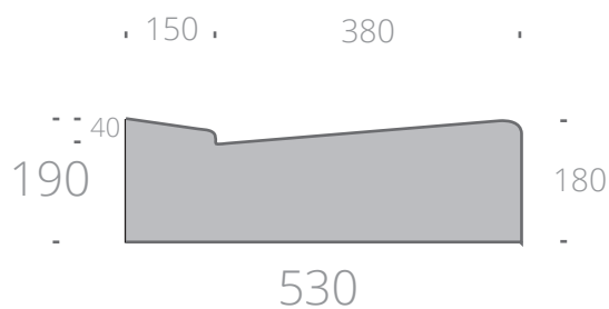
Cutdown Kerb and Channel
