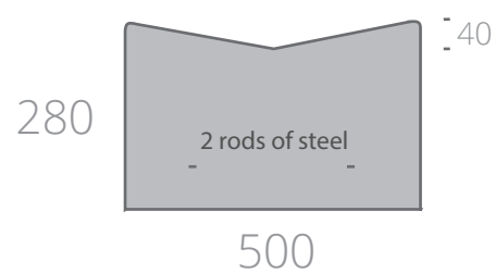
Hillside V - Channel (500mm) with steel
