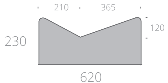
Hillside V - Channel (620mm)
