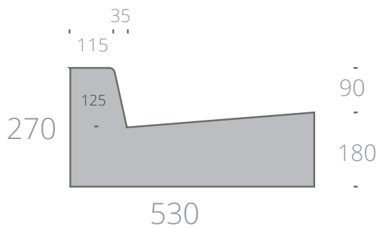
Sloping Kerb and Channel
