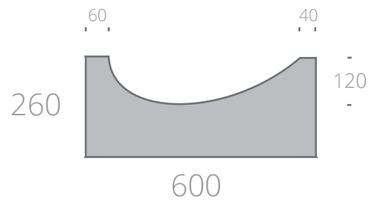
Off Set 600mm Dish Channel
