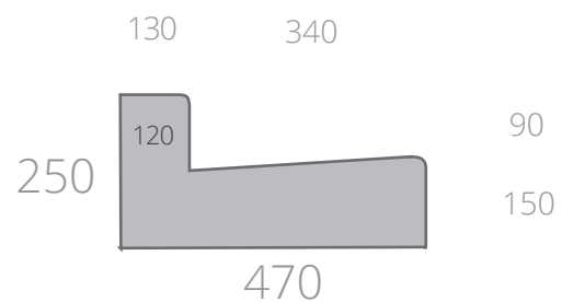
Timaru Kerb and Channel
