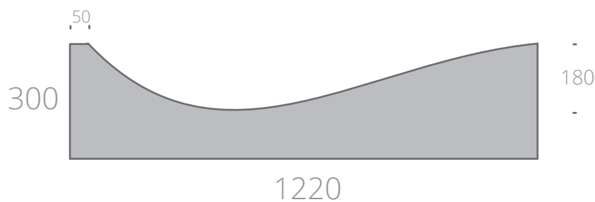
1220mm Dish Channel
