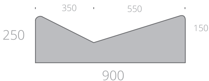
Hillside V - Channel (900mm)
