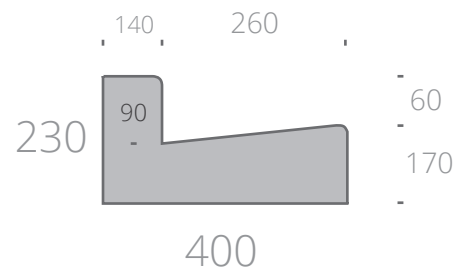
Small Kerb and Channel
