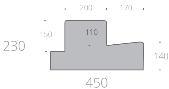
Pegasus Kerb & Channel
